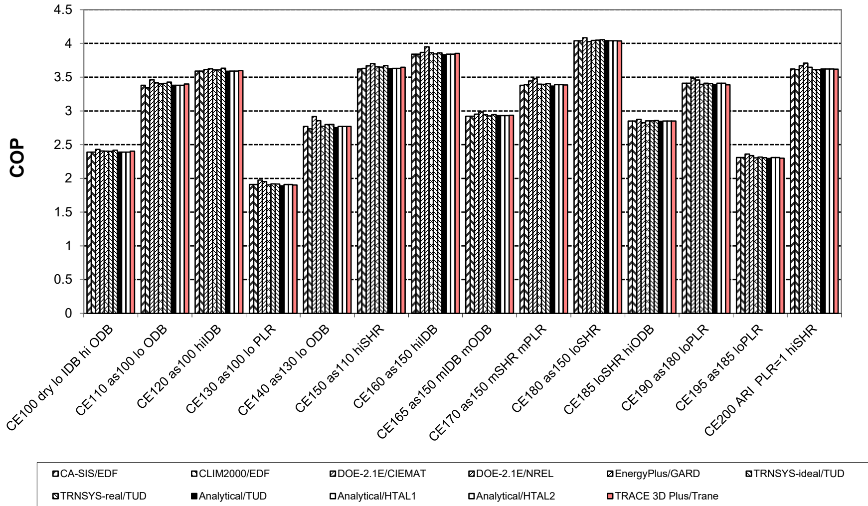
Figure B16.5.1-1. HVAC BESTEST: Mean COP
