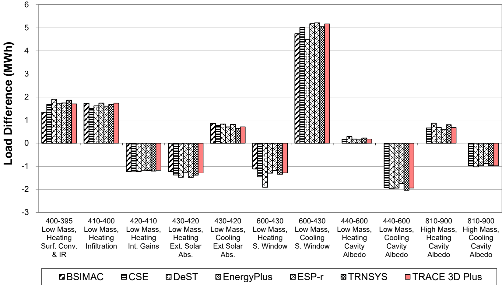
Figure B8-54. In-Depth: Cases 395 to 600, 810 to 900 (Delta) Annual Heating and Sensible Cooling
