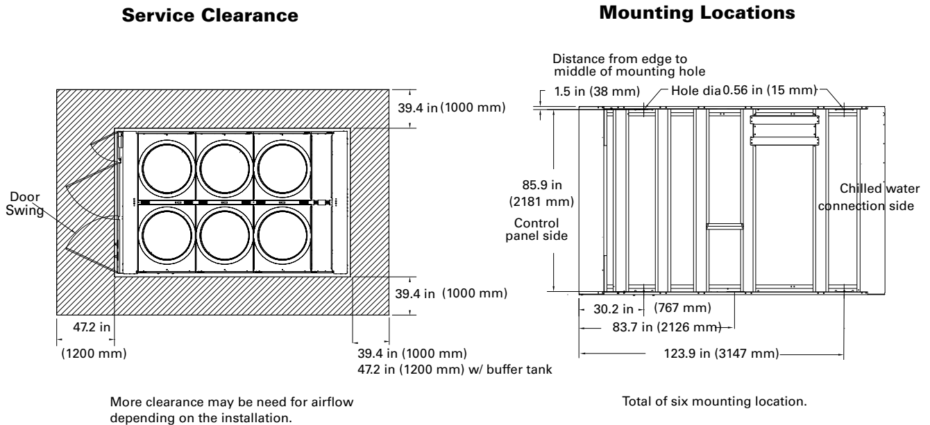
Figure 10. CGAM 80 and 90 (compact version) - service clearances and mounting locations
