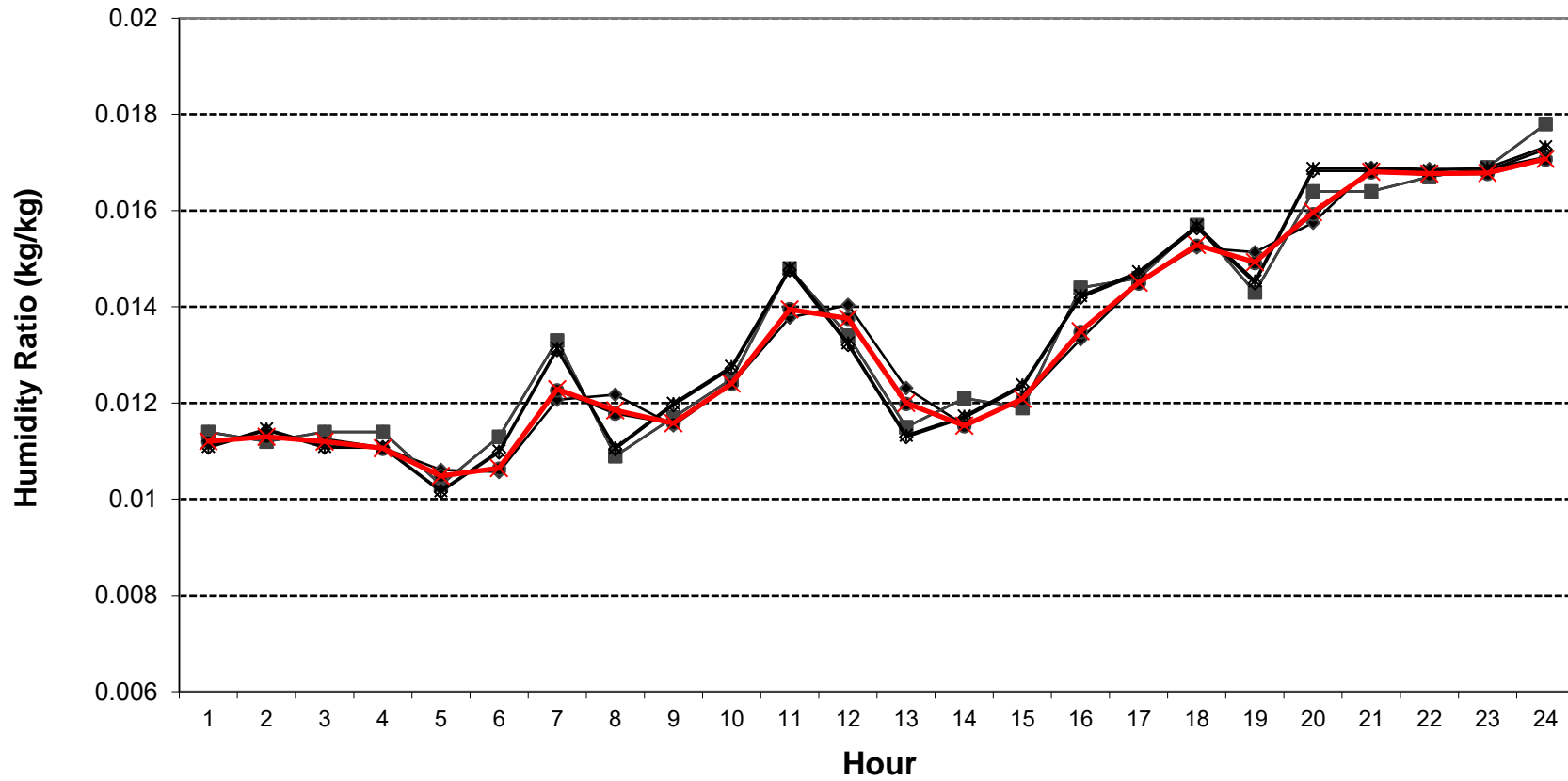
Figure B16.5.2-52. HVAC BESTEST: CE300 June 28 Hourly OHR
